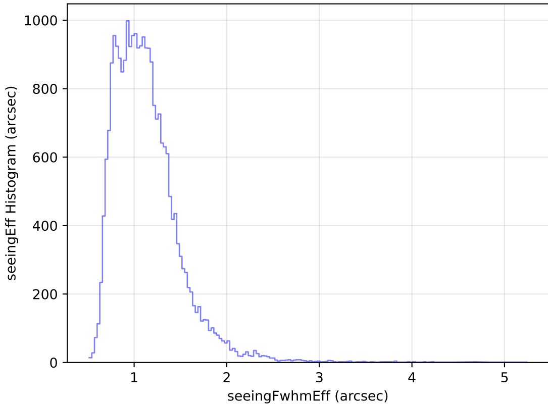
too_elab_r256_d3_ugrizy_v3.4_10yrs Yr 1 g band: seeingEff Histogram
