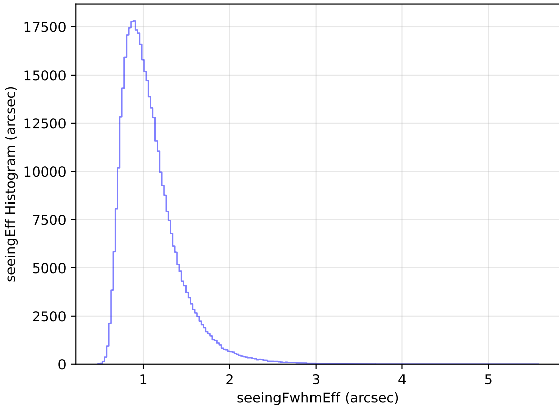
too_elab_r256_d3_ugrizy_v3.4_10yrs WFD z band: seeingEff Histogram
