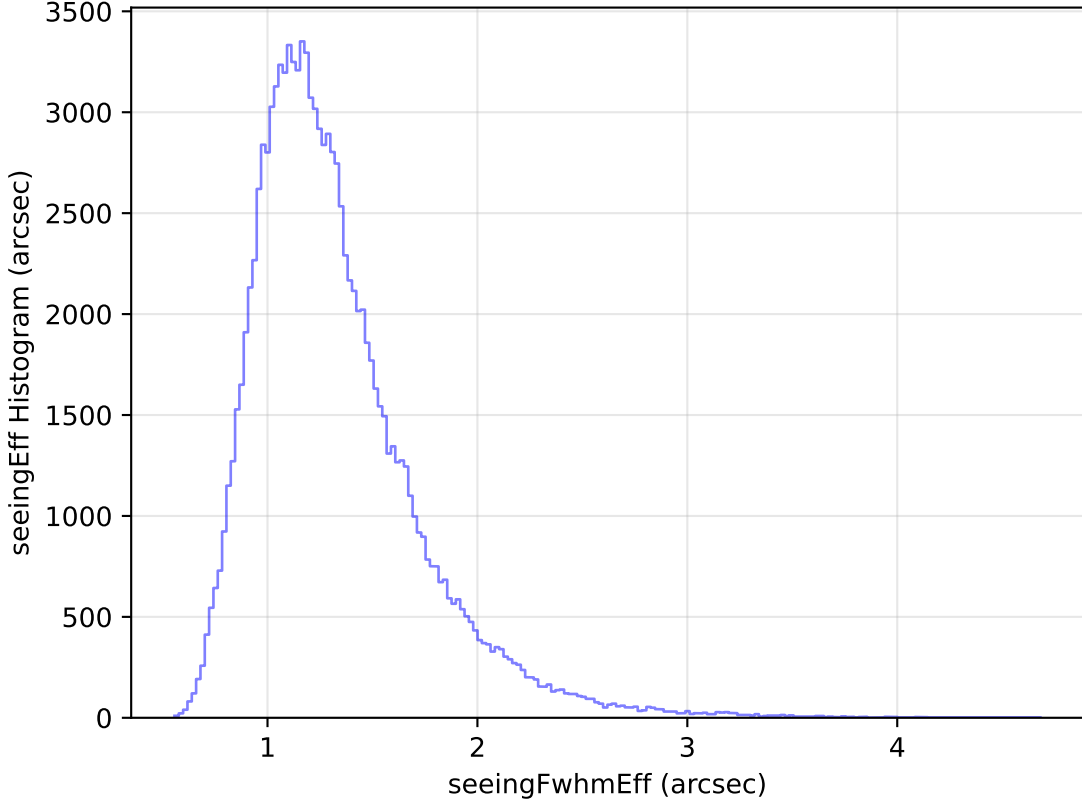
too_elab_r256_d3_ugrizy_v3.4_10yrs WFD u band: seeingEff Histogram
