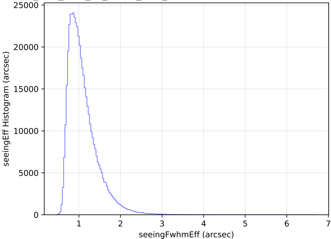
too_elab_r256_d3_ugrizy_v3.4_10yrs WFD i band: seeingEff Histogram
