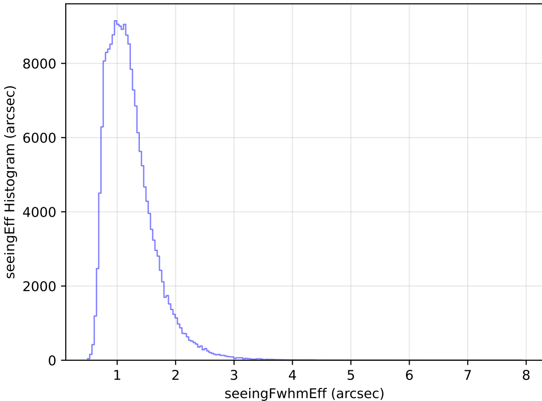
too_elab_r256_d3_ugrizy_v3.4_10yrs WFD g band: seeingEff Histogram
