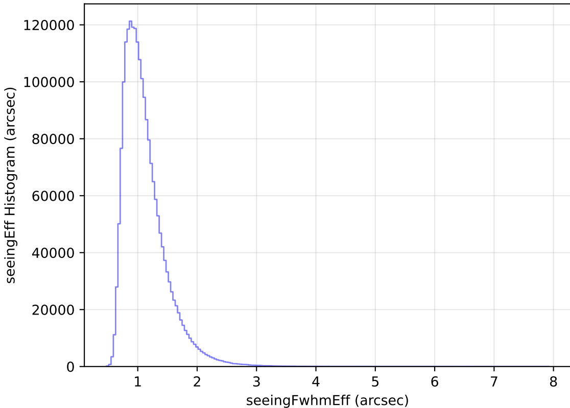
too_elab_r256_d3_ugrizy_v3.4_10yrs WFD all bands: seeingEff Histogram
