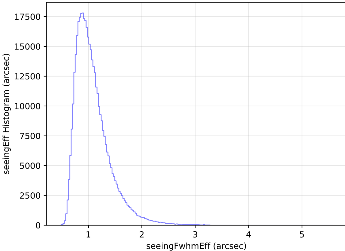
too_elab_r256_d3_ugrizy_v3.4_10yrs All sky z band: seeingEff Histogram
