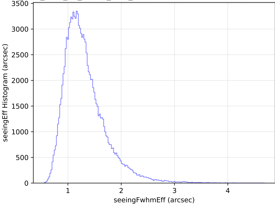
too_elab_r256_d3_ugrizy_v3.4_10yrs All sky u band: seeingEff Histogram
