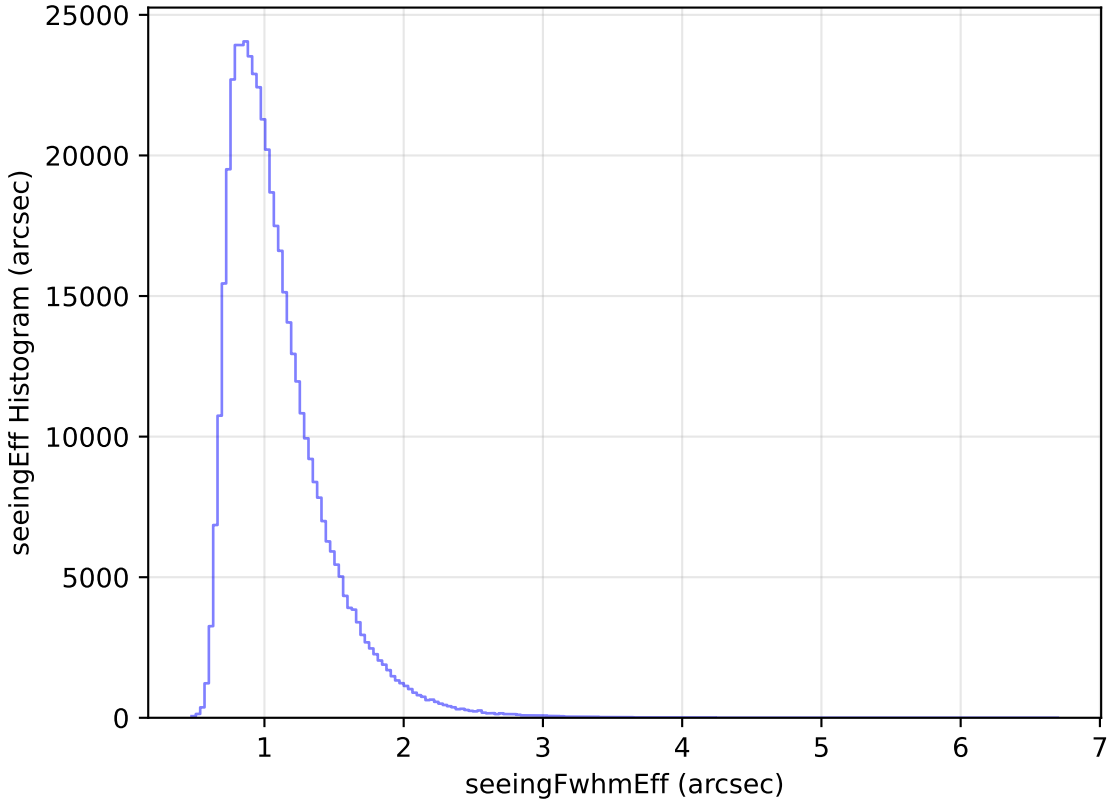
too_elab_r256_d3_ugrizy_v3.4_10yrs All sky i band: seeingEff Histogram
