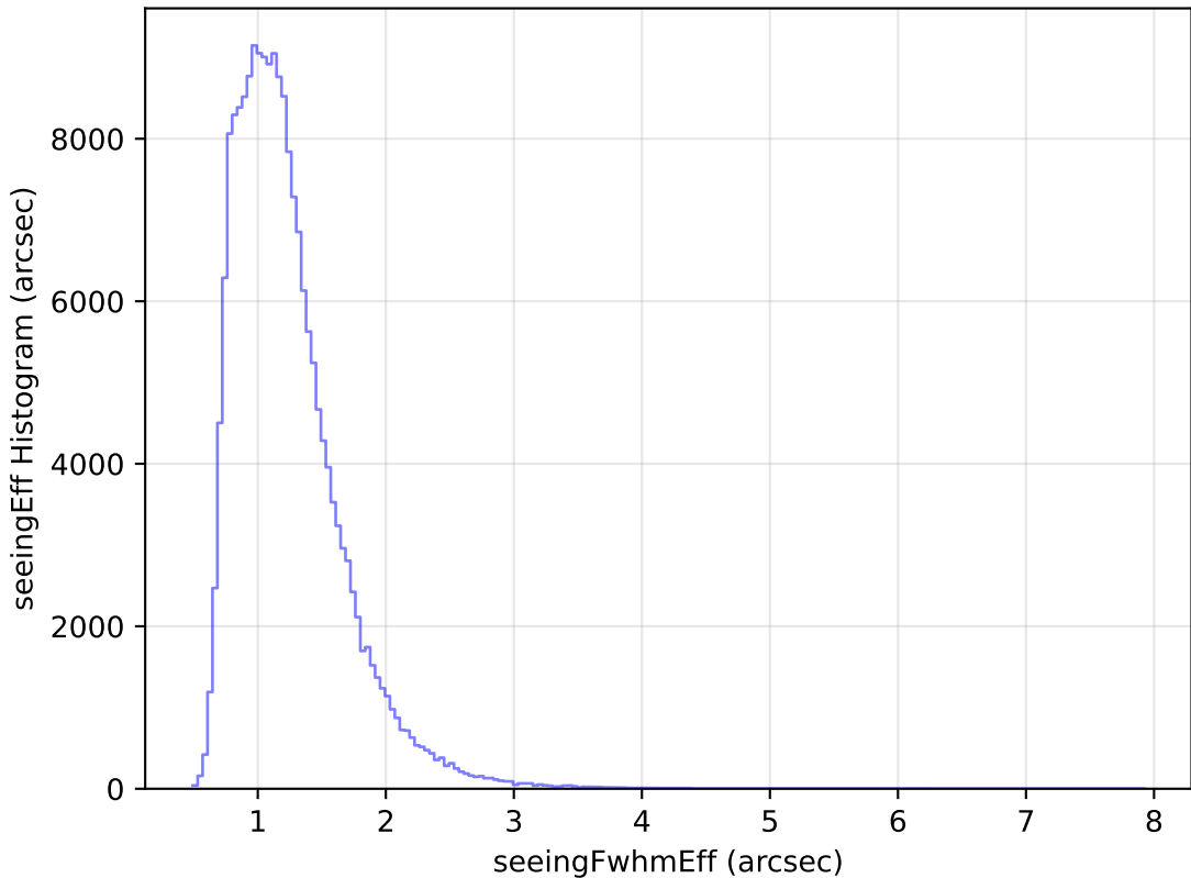
too_elab_r256_d3_ugrizy_v3.4_10yrs All sky g band: seeingEff Histogram
