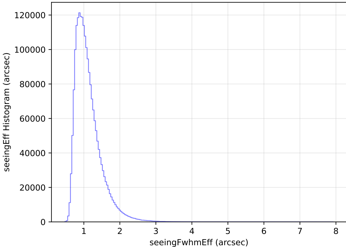
too_elab_r256_d3_ugrizy_v3.4_10yrs All sky all bands: seeingEff Histogram
