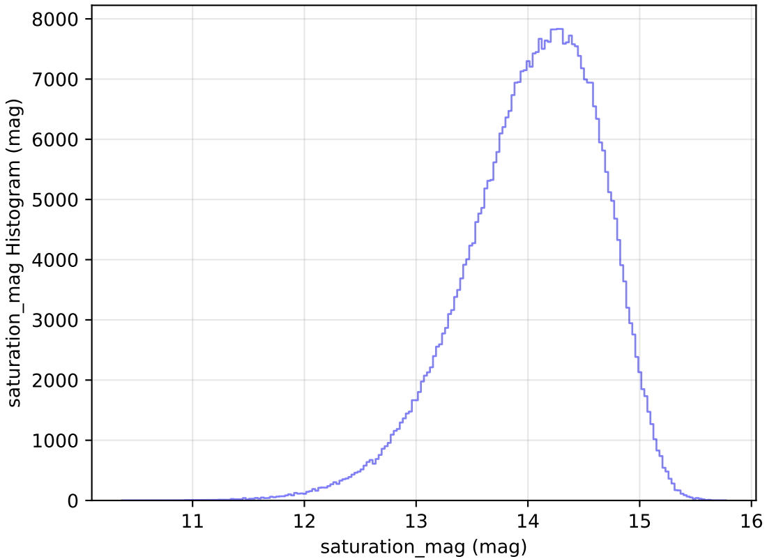
too_elab_r256_d3_ugrizy_v3.4_10yrs WFD z band: saturation_mag Histogram
