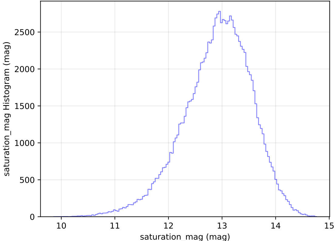
too_elab_r256_d3_ugrizy_v3.4_10yrs WFD u band: saturation_mag Histogram
