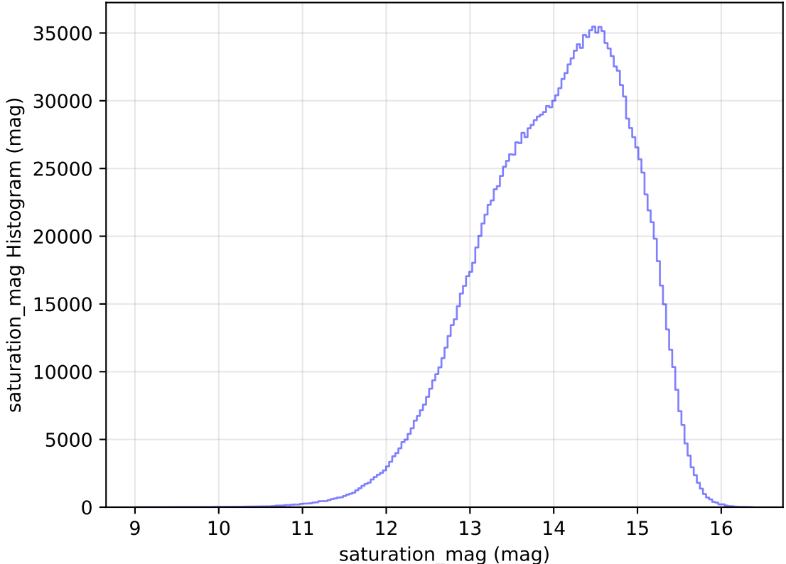
too_elab_r256_d3_ugrizy_v3.4_10yrs WFD all bands: saturation_mag Histogram
