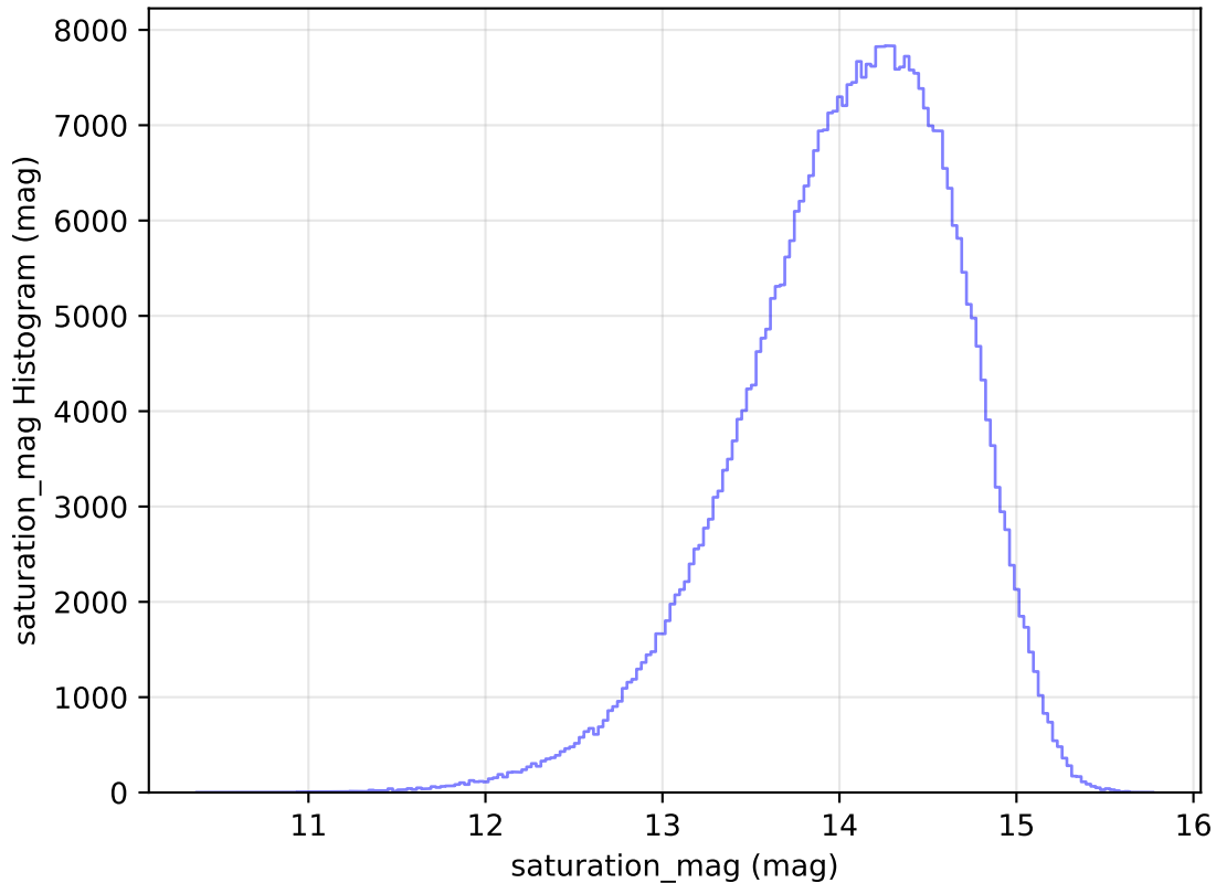
too_elab_r256_d3_ugrizy_v3.4_10yrs All sky z band: saturation_mag Histogram
