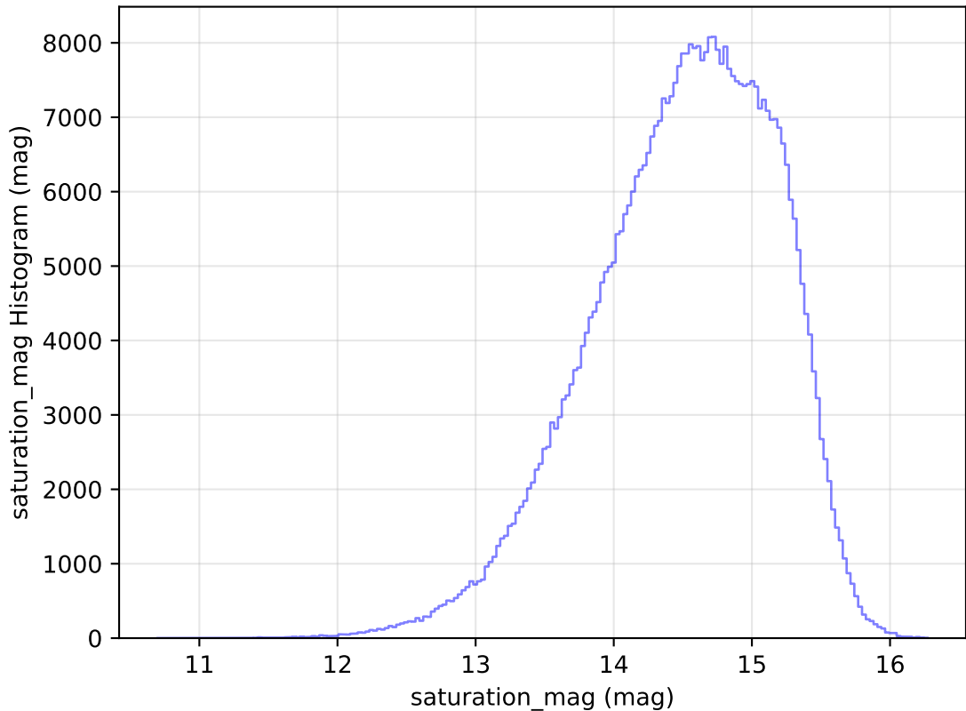
too_elab_r256_d3_ugrizy_v3.4_10yrs All sky r band: saturation_mag Histogram
