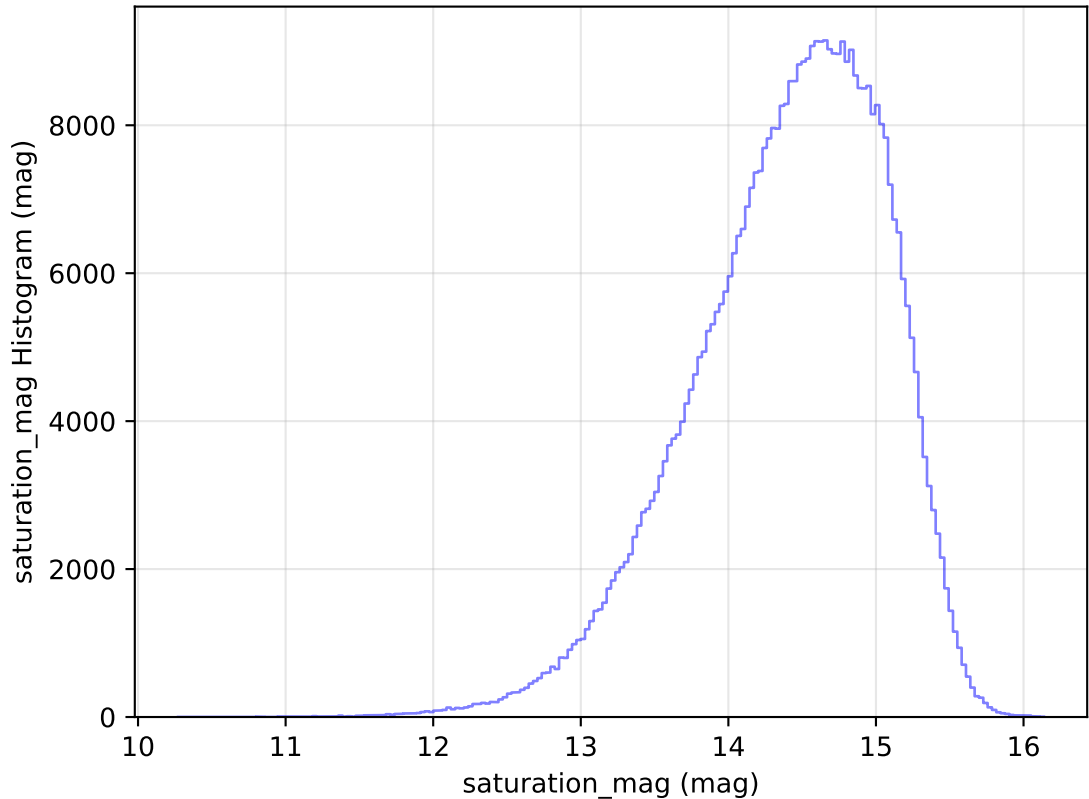
too_elab_r256_d3_ugrizy_v3.4_10yrs All sky i band: saturation_mag Histogram
