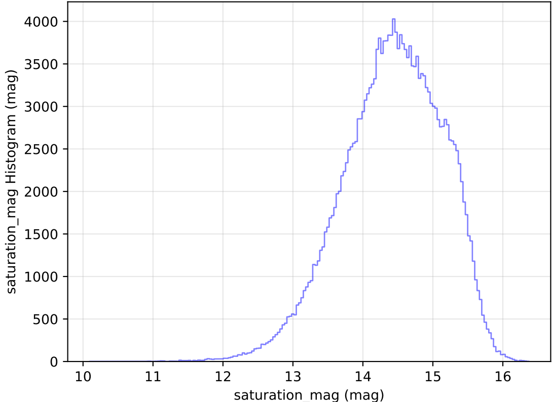
too_elab_r256_d3_ugrizy_v3.4_10yrs All sky g band: saturation_mag Histogram
