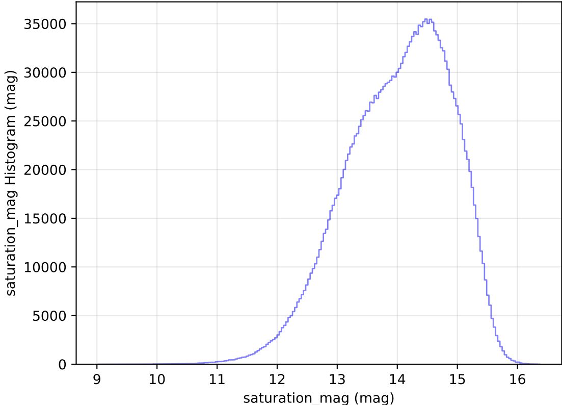
too_elab_r256_d3_ugrizy_v3.4_10yrs All sky all bands: saturation_mag Histogram
