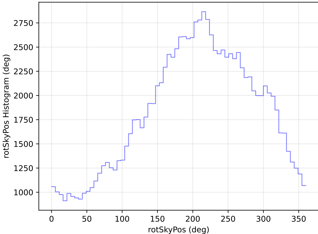
too_elab_r256_d3_ugrizy_v3.4_10yrs All sky u band: rotSkyPos Histogram
