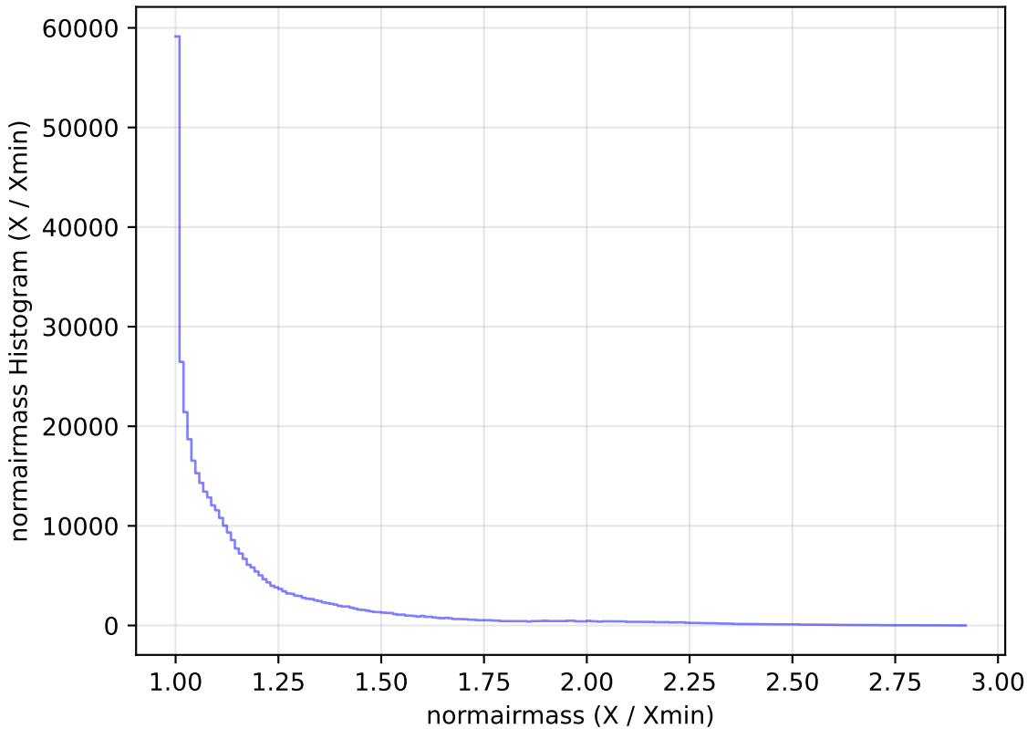
too_elab_r256_d3_ugrizy_v3.4_10yrs WFD z band: normairmass Histogram
