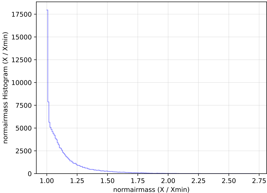
too_elab_r256_d3_ugrizy_v3.4_10yrs WFD u band: normairmass Histogram
