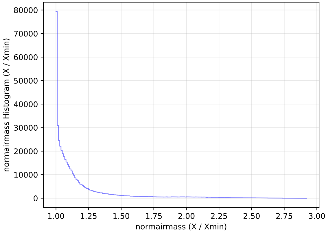
too_elab_r256_d3_ugrizy_v3.4_10yrs WFD i band: normairmass Histogram
