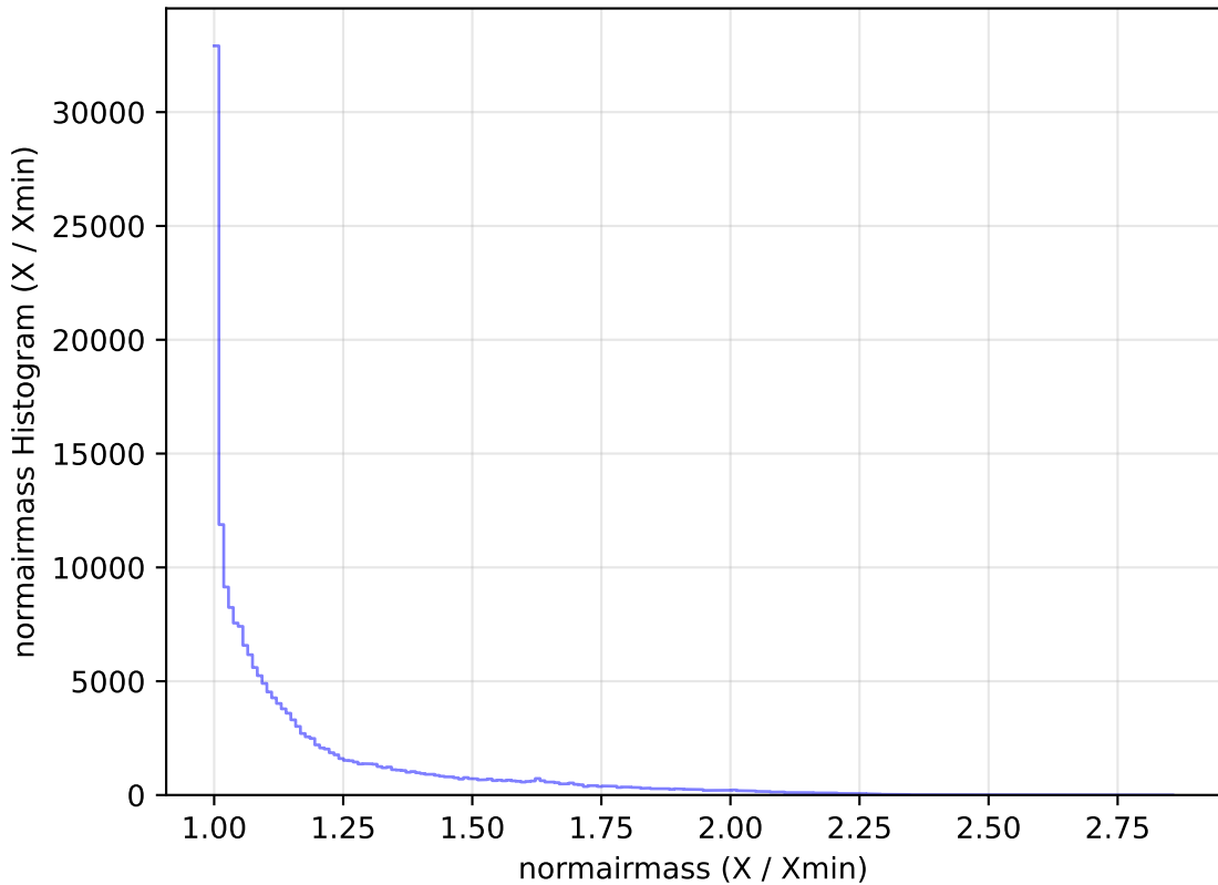
too_elab_r256_d3_ugrizy_v3.4_10yrs WFD g band: normairmass Histogram
