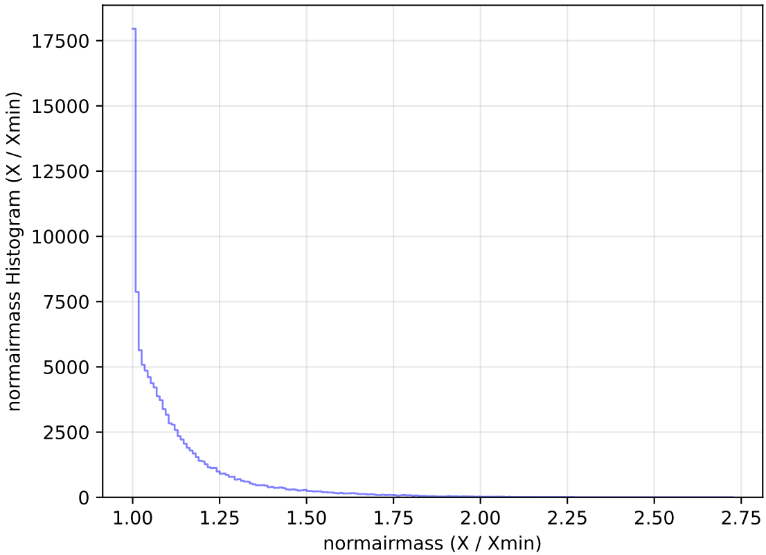
too_elab_r256_d3_ugrizy_v3.4_10yrs All sky u band: normairmass Histogram
