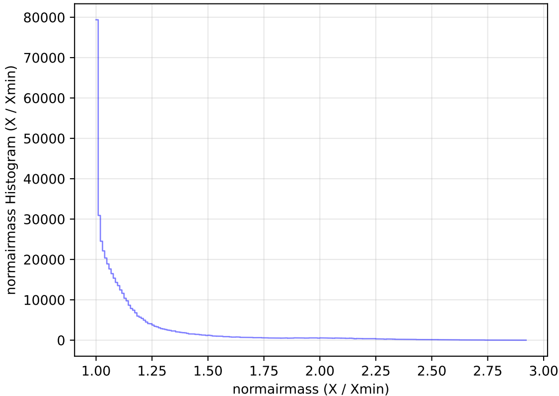
too_elab_r256_d3_ugrizy_v3.4_10yrs All sky i band: normairmass Histogram
