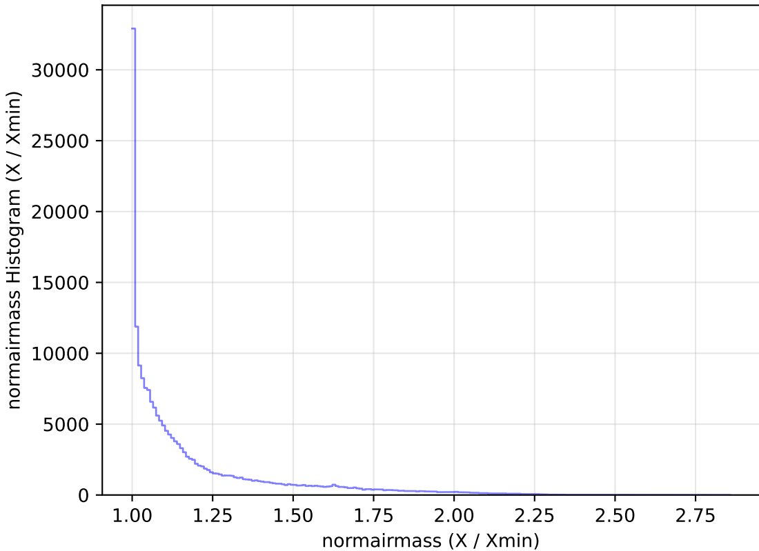
too_elab_r256_d3_ugrizy_v3.4_10yrs All sky g band: normairmass Histogram
