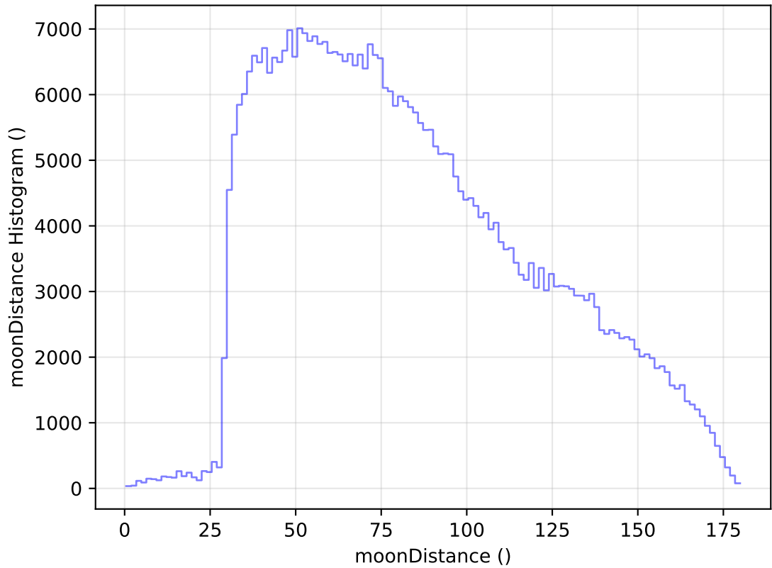
too_elab_r256_d3_ugrizy_v3.4_10yrs WFD z band: moonDistance Histogram
