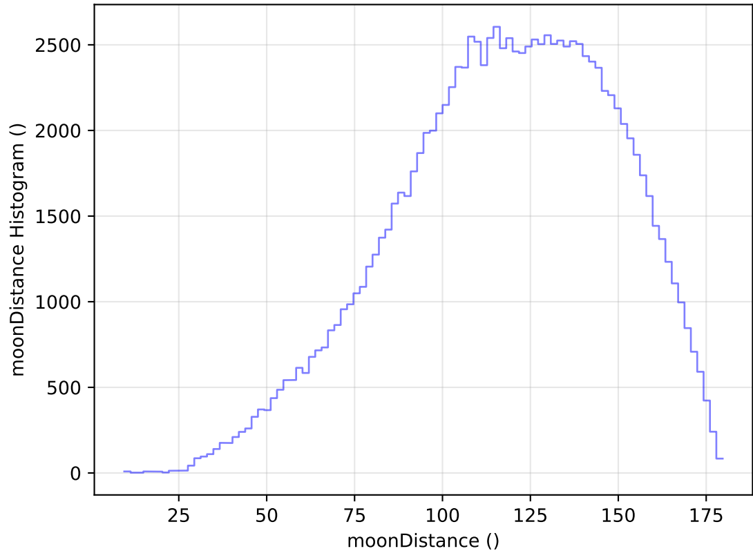
too_elab_r256_d3_ugrizy_v3.4_10yrs WFD u band: moonDistance Histogram
