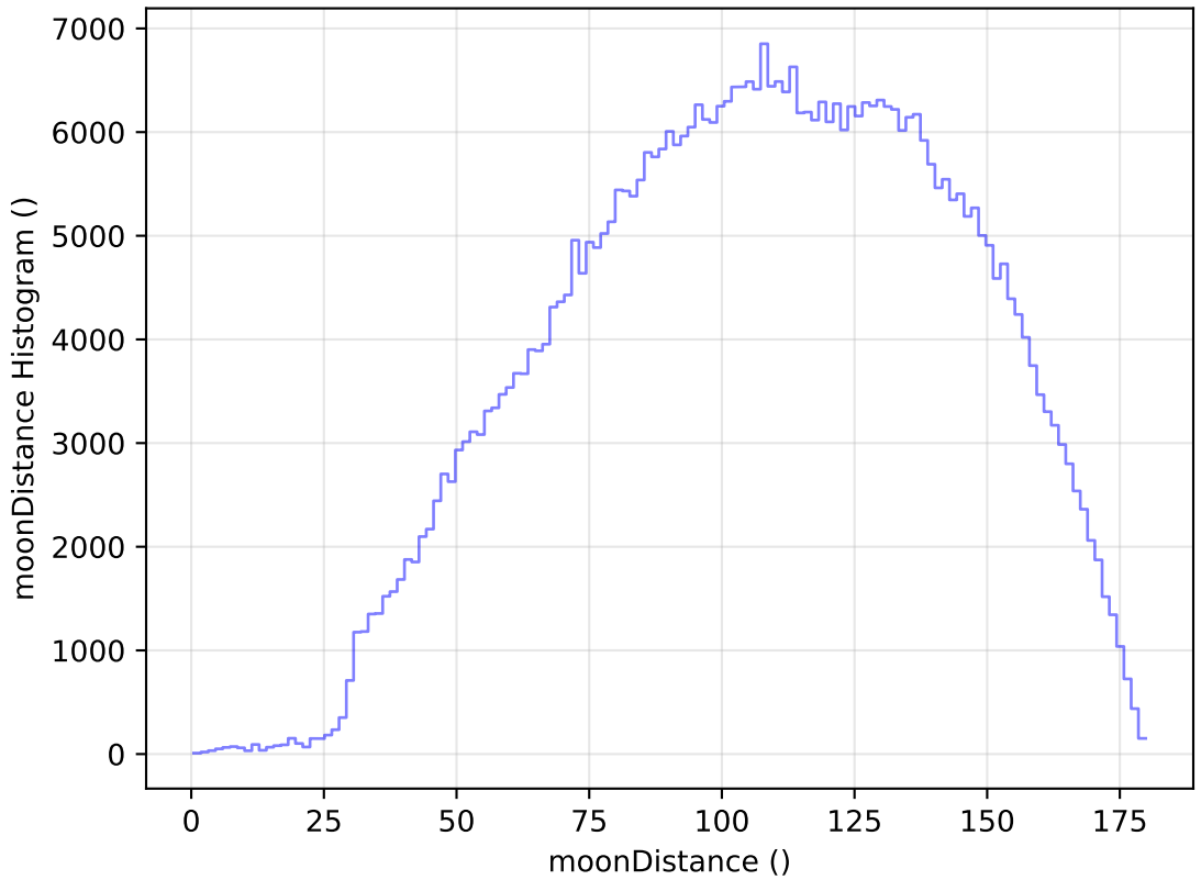
too_elab_r256_d3_ugrizy_v3.4_10yrs WFD r band: moonDistance Histogram
