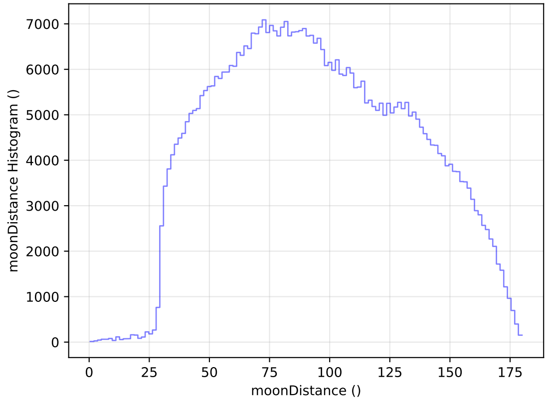
too_elab_r256_d3_ugrizy_v3.4_10yrs WFD i band: moonDistance Histogram
