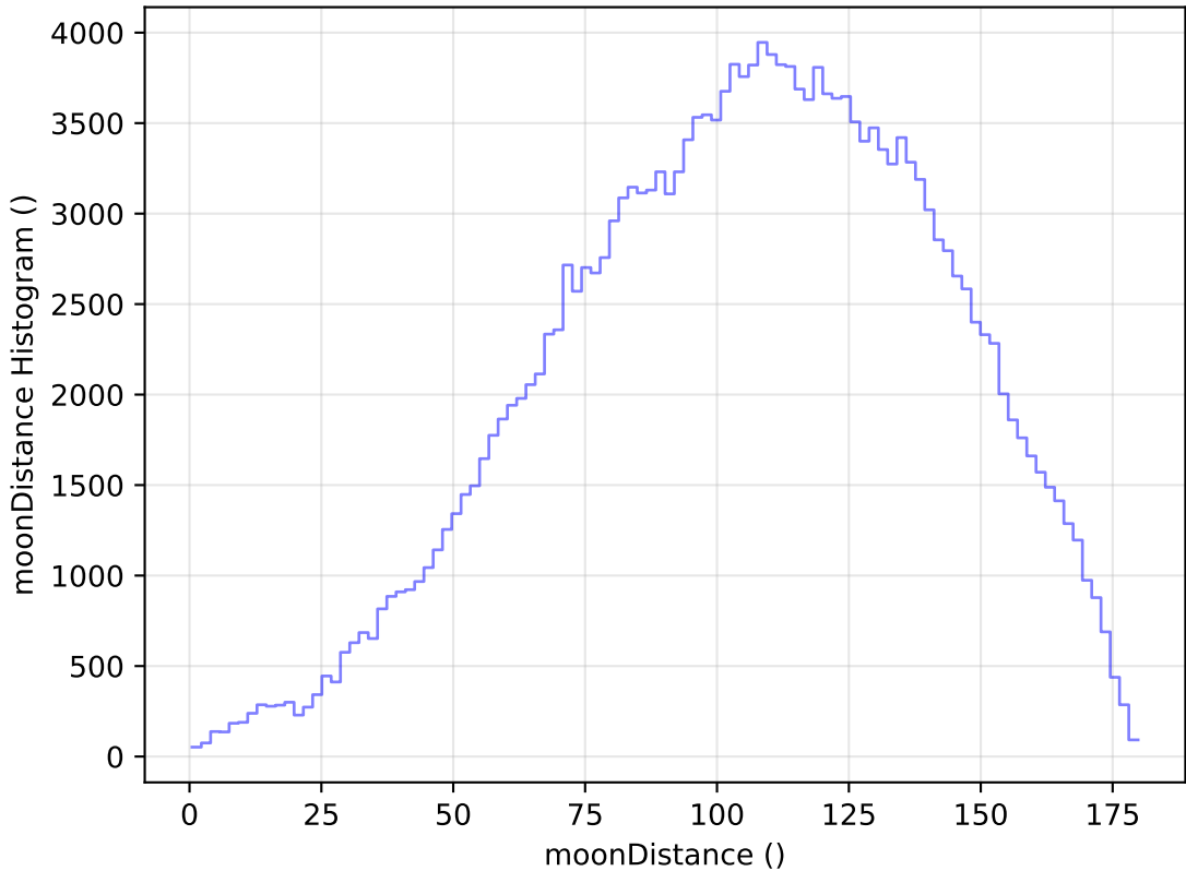
too_elab_r256_d3_ugrizy_v3.4_10yrs WFD g band: moonDistance Histogram
