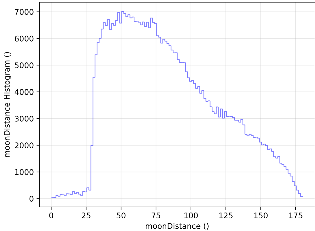
too_elab_r256_d3_ugrizy_v3.4_10yrs All sky z band: moonDistance Histogram
