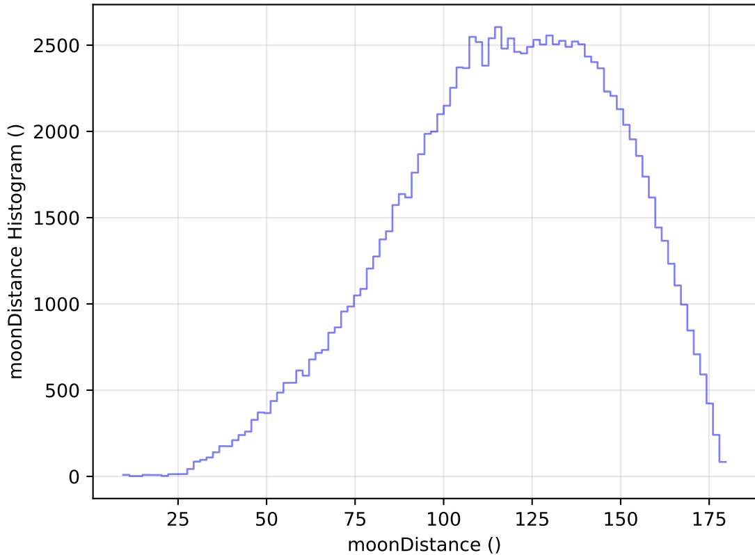
too_elab_r256_d3_ugrizy_v3.4_10yrs All sky u band: moonDistance Histogram
