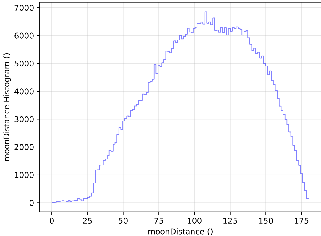
too_elab_r256_d3_ugrizy_v3.4_10yrs All sky r band: moonDistance Histogram
