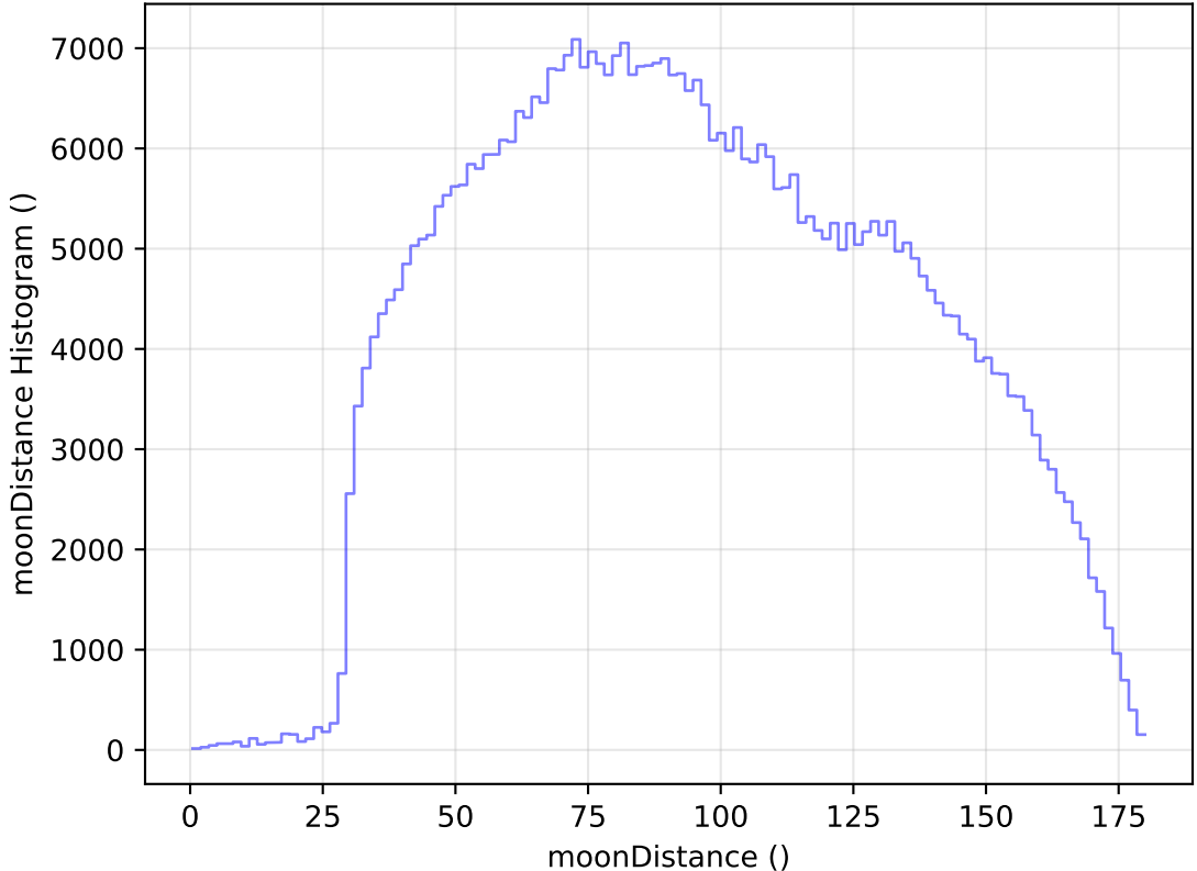
too_elab_r256_d3_ugrizy_v3.4_10yrs All sky i band: moonDistance Histogram
