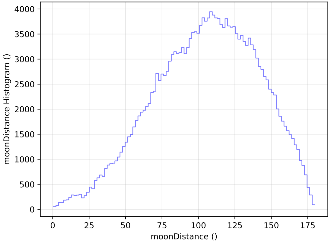
too_elab_r256_d3_ugrizy_v3.4_10yrs All sky g band: moonDistance Histogram
