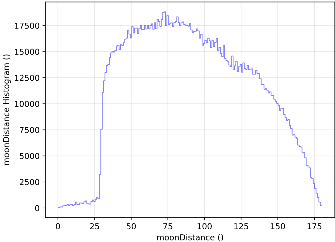
too_elab_r256_d3_ugrizy_v3.4_10yrs All sky all bands: moonDistance Histogram
