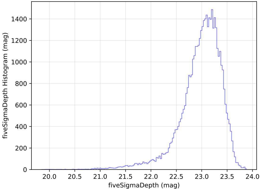
too_elab_r256_d3_ugrizy_v3.4_10yrs Yr 1 z band: fiveSigmaDepth Histogram
