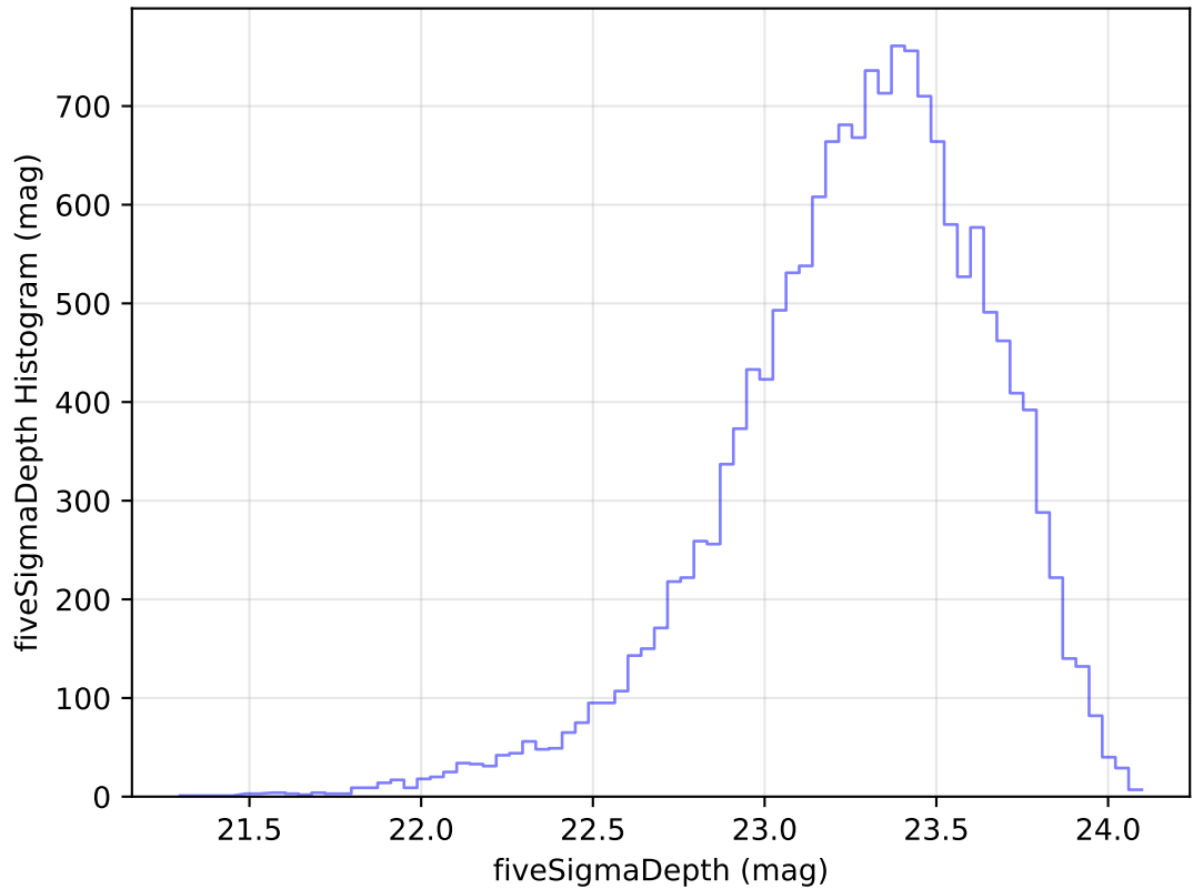
too_elab_r256_d3_ugrizy_v3.4_10yrs Yr 1 u band: fiveSigmaDepth Histogram
