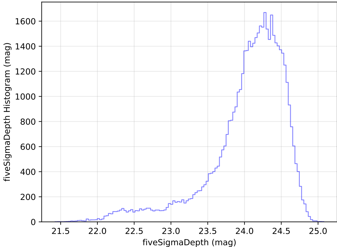
too_elab_r256_d3_ugrizy_v3.4_10yrs Yr 1 r band: fiveSigmaDepth Histogram
