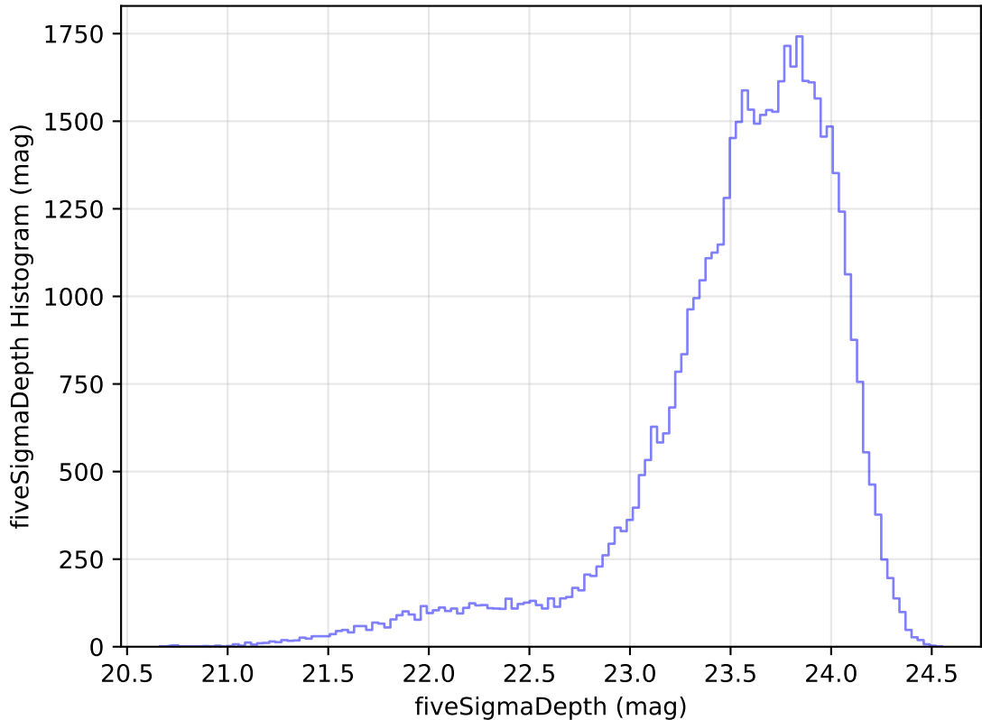
too_elab_r256_d3_ugrizy_v3.4_10yrs Yr 1 i band: fiveSigmaDepth Histogram
