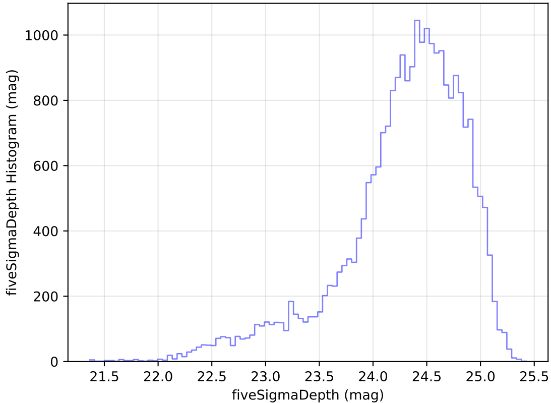
too_elab_r256_d3_ugrizy_v3.4_10yrs Yr 1 g band: fiveSigmaDepth Histogram
