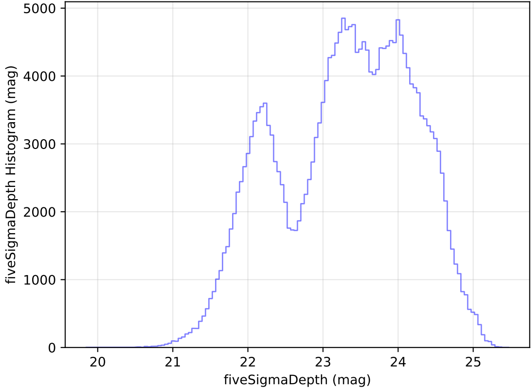
too_elab_r256_d3_ugrizy_v3.4_10yrs Yr 1 all bands: fiveSigmaDepth Histogram
