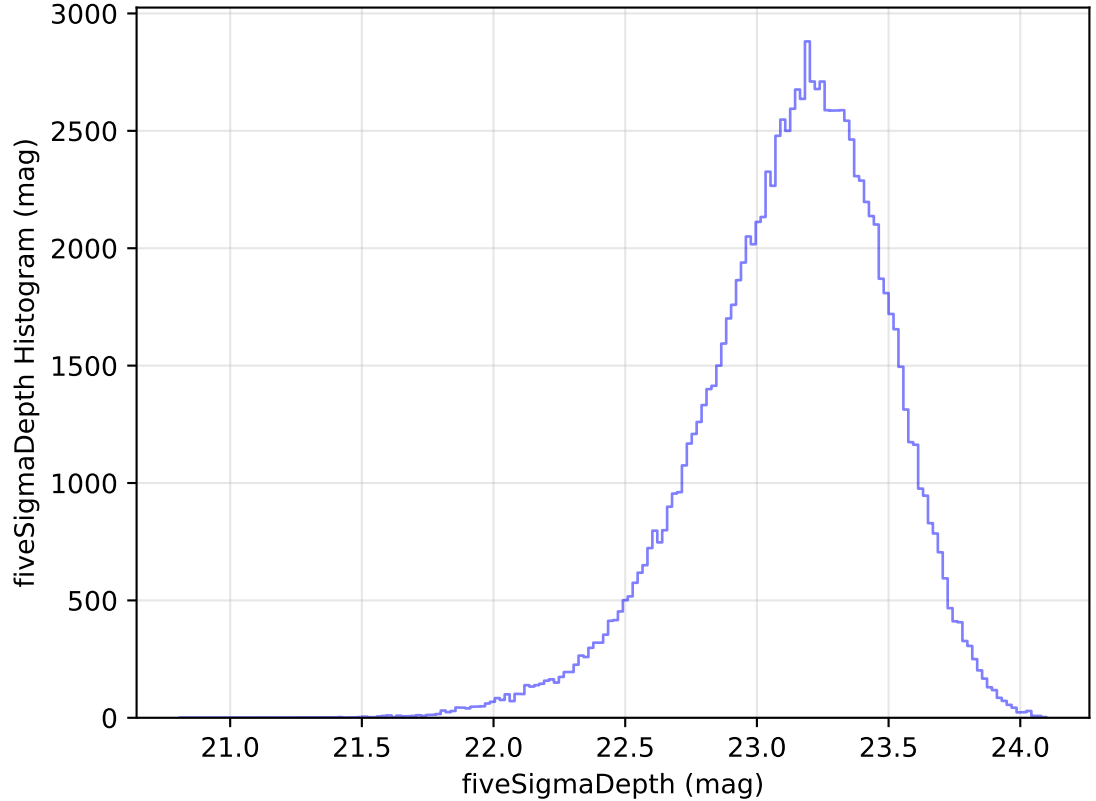
too_elab_r256_d3_ugrizy_v3.4_10yrs WFD u band: fiveSigmaDepth Histogram
