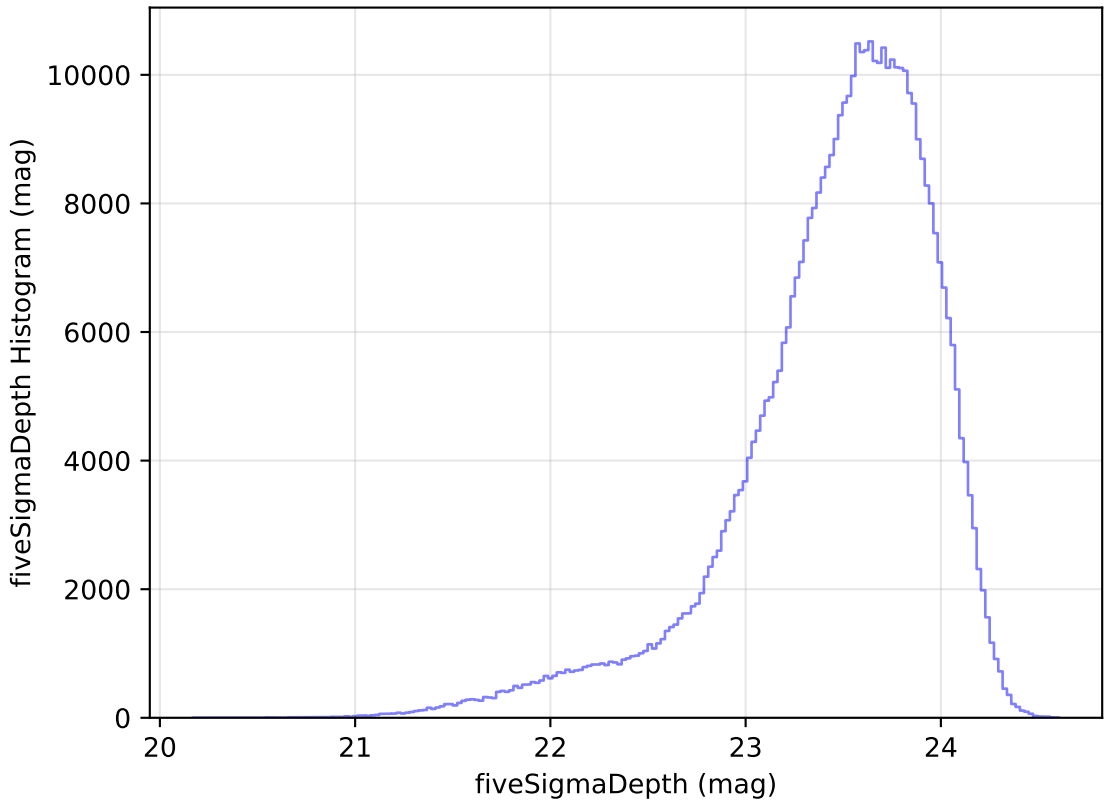
too_elab_r256_d3_ugrizy_v3.4_10yrs WFD i band: fiveSigmaDepth Histogram
