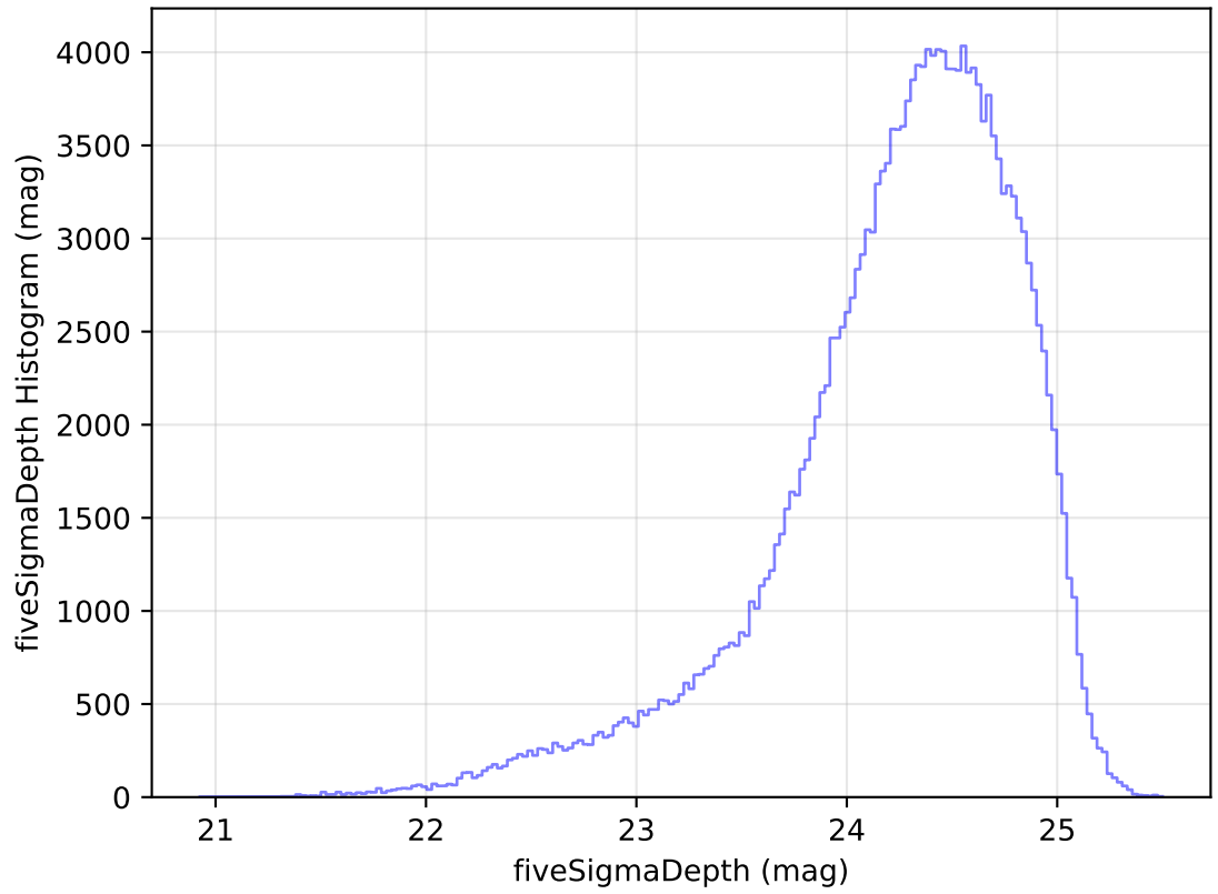
too_elab_r256_d3_ugrizy_v3.4_10yrs WFD g band: fiveSigmaDepth Histogram
