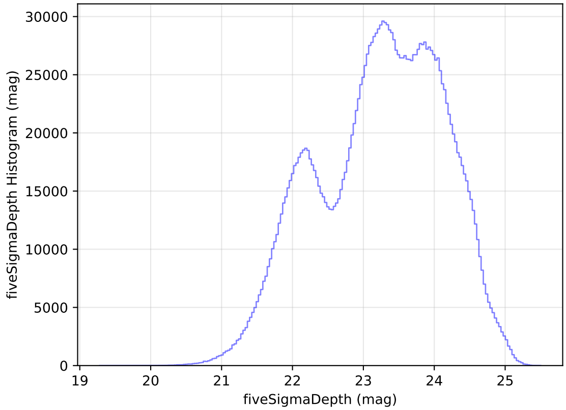
too_elab_r256_d3_ugrizy_v3.4_10yrs WFD all bands: fiveSigmaDepth Histogram
