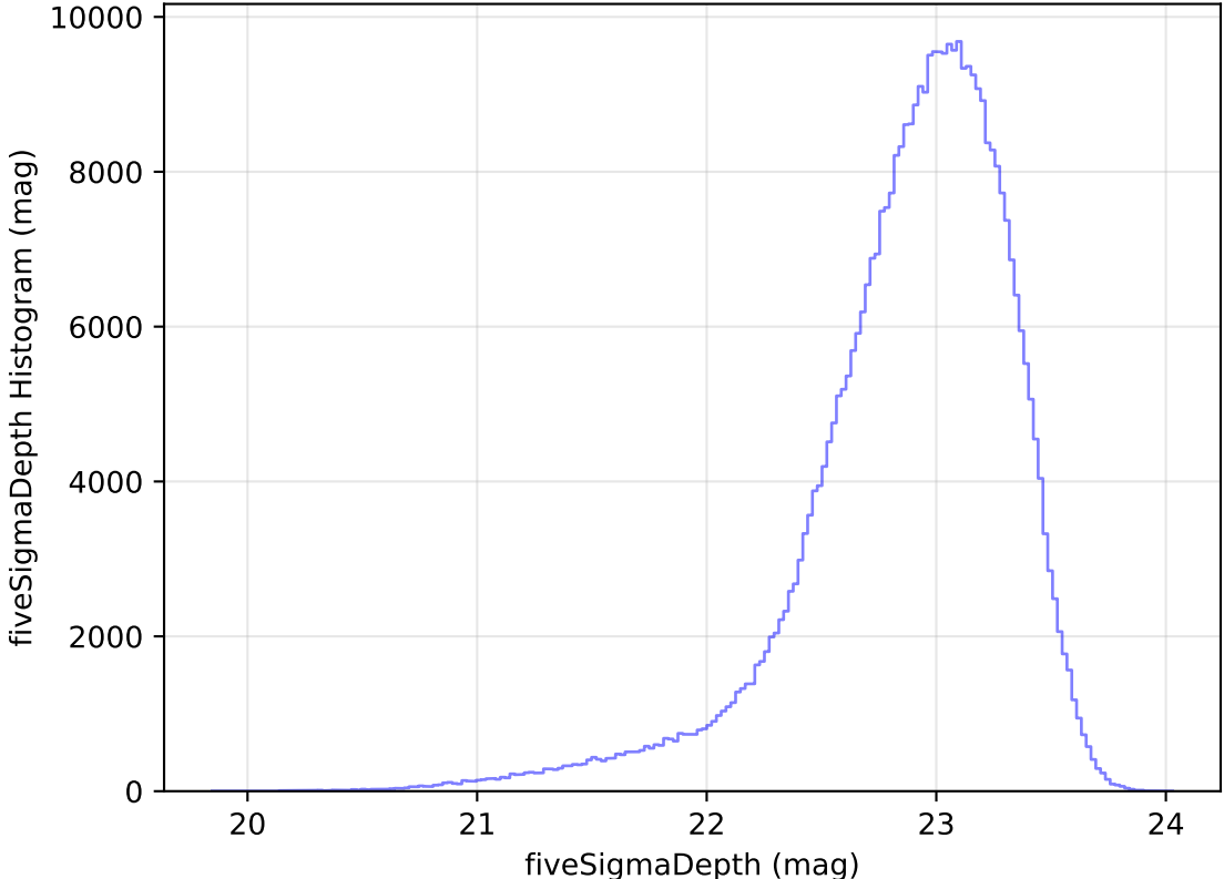
too_elab_r256_d3_ugrizy_v3.4_10yrs All sky z band: fiveSigmaDepth Histogram
