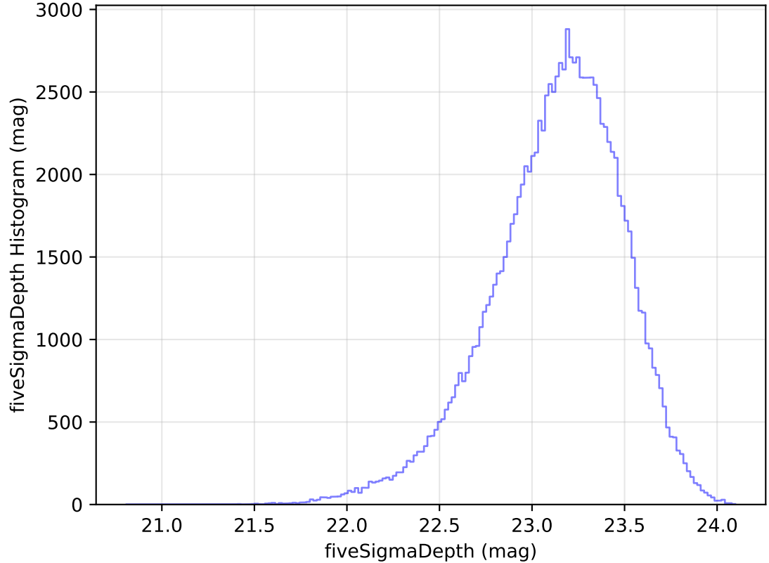
too_elab_r256_d3_ugrizy_v3.4_10yrs All sky u band: fiveSigmaDepth Histogram
